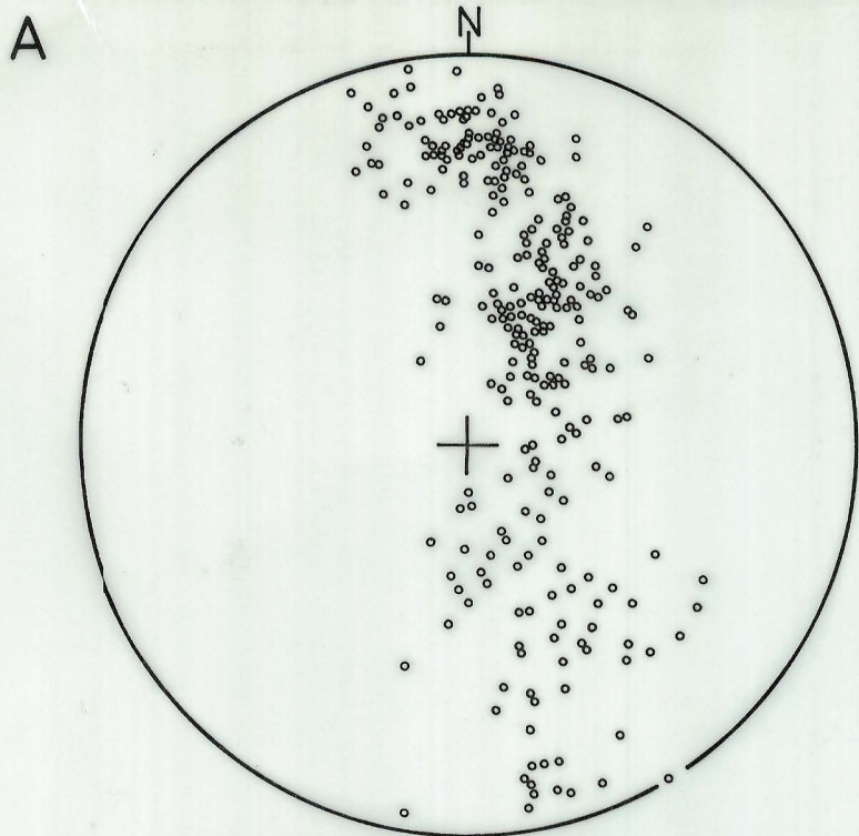
271 Poles to S_0
