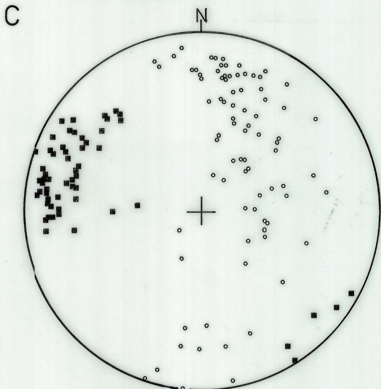
◦ Poles to S_1 ■ F_1 Hinge
