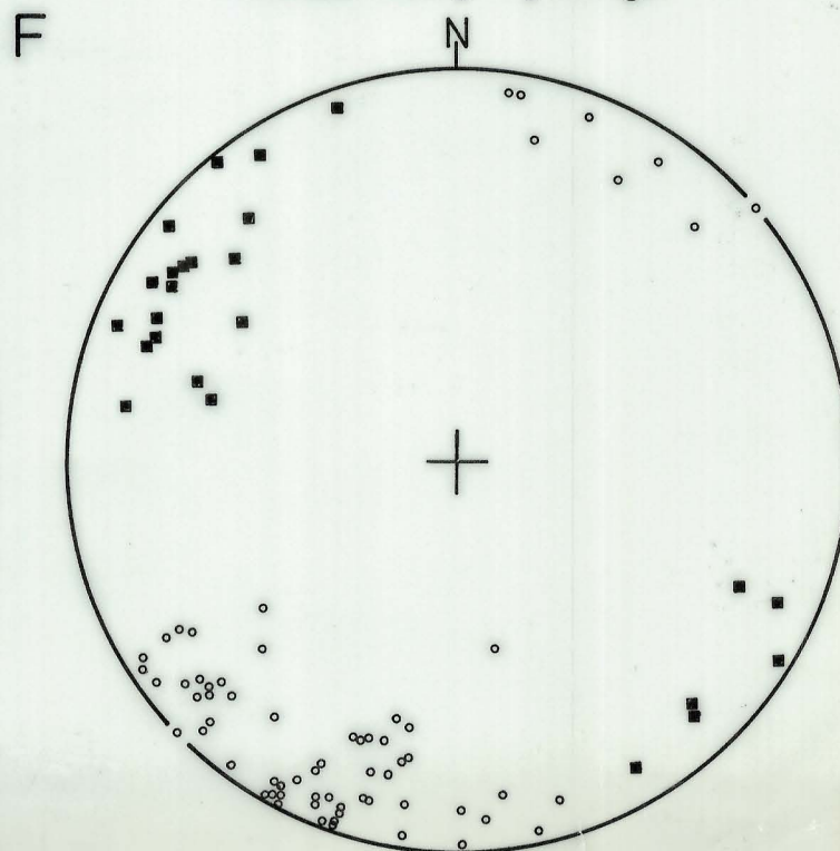
◦ Poles to S_4 ■ F_4 Hinge
