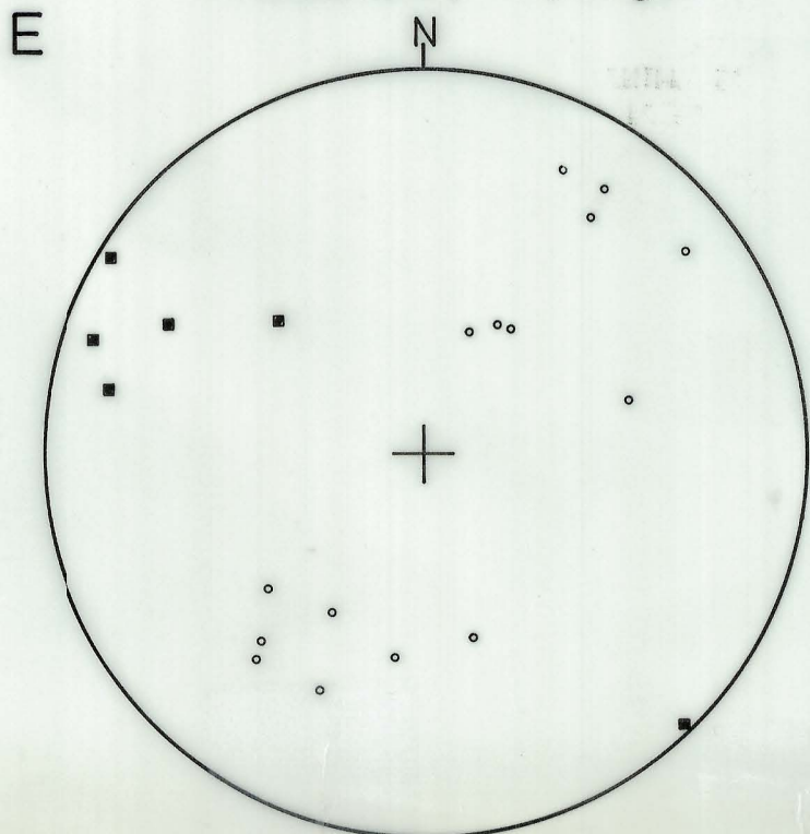
◦ Poles to S_3 ■ F_3 Hinge
