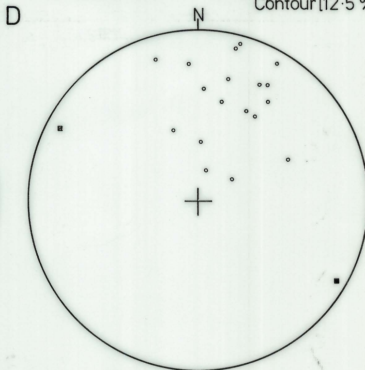
◦ Poles to S_2 ■ F_2 Hinge
