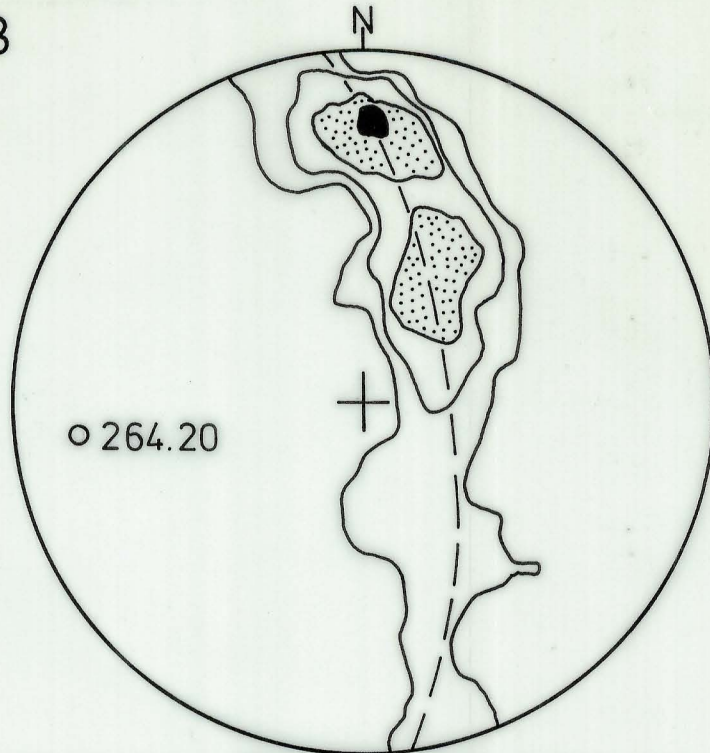
A Contoured at 95%, 50%, 25%, 12.5% of Maximum Contour [12.5 %]
