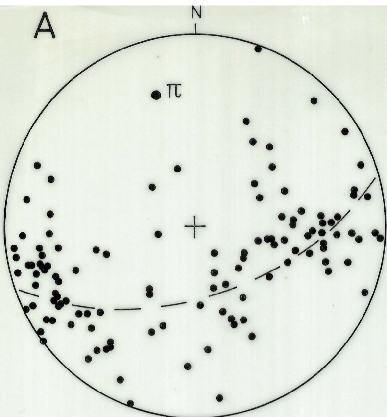
POLES TO ALL COMPOSITIONAL LAYERS. 119 POINTS.
