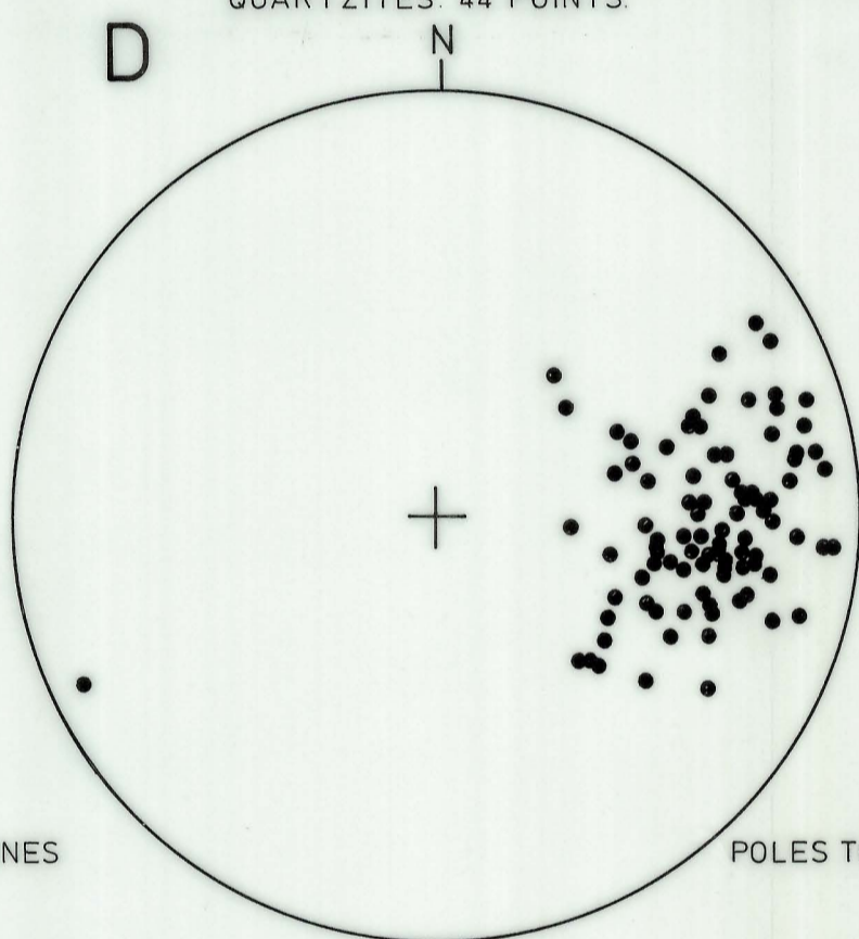
POLES TO COMPOSITIONAL LAYERS. FLAGGY QUARTZITES. 44 POINTS.
