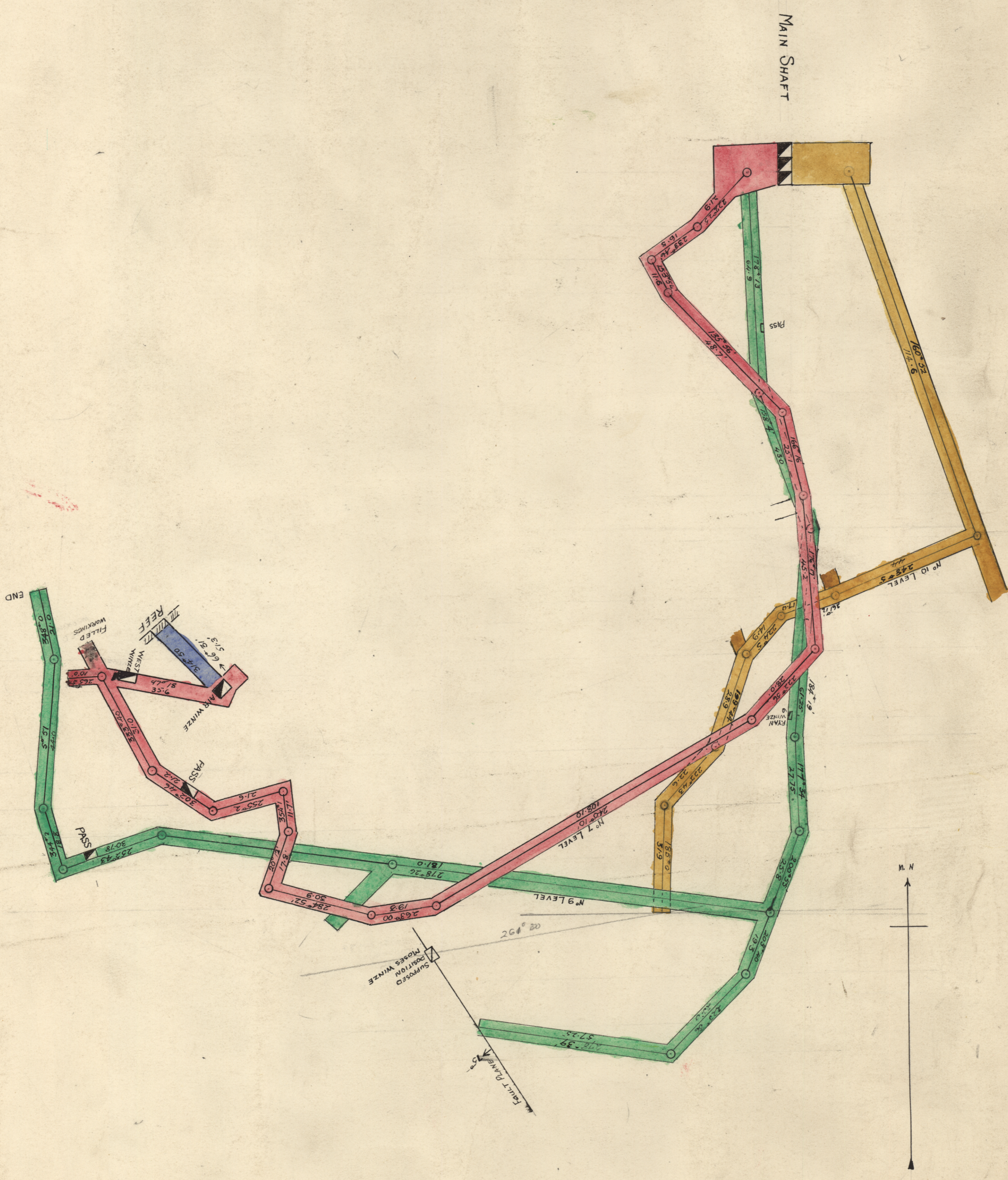
— GOLDEN GATE CONSOLIDATED MINE — — PLAN OF PORTION OF N os 7, 9 & 10 LEVELS — — SCALE 1 INCH = 20 FEET —
