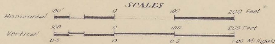
GEOPHYSICAL SURVEY AT ZEEHAN TASMANIA MARIPOSA AREA VERTICAL SECTIONS THROUGH DIAMOND DRILL HOLES SHOWING RELATIONS TO GRAVITY ANOMALIES.
