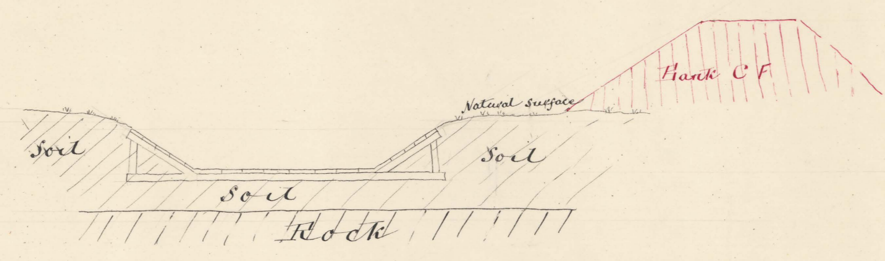
Cross Section midway between D & C
