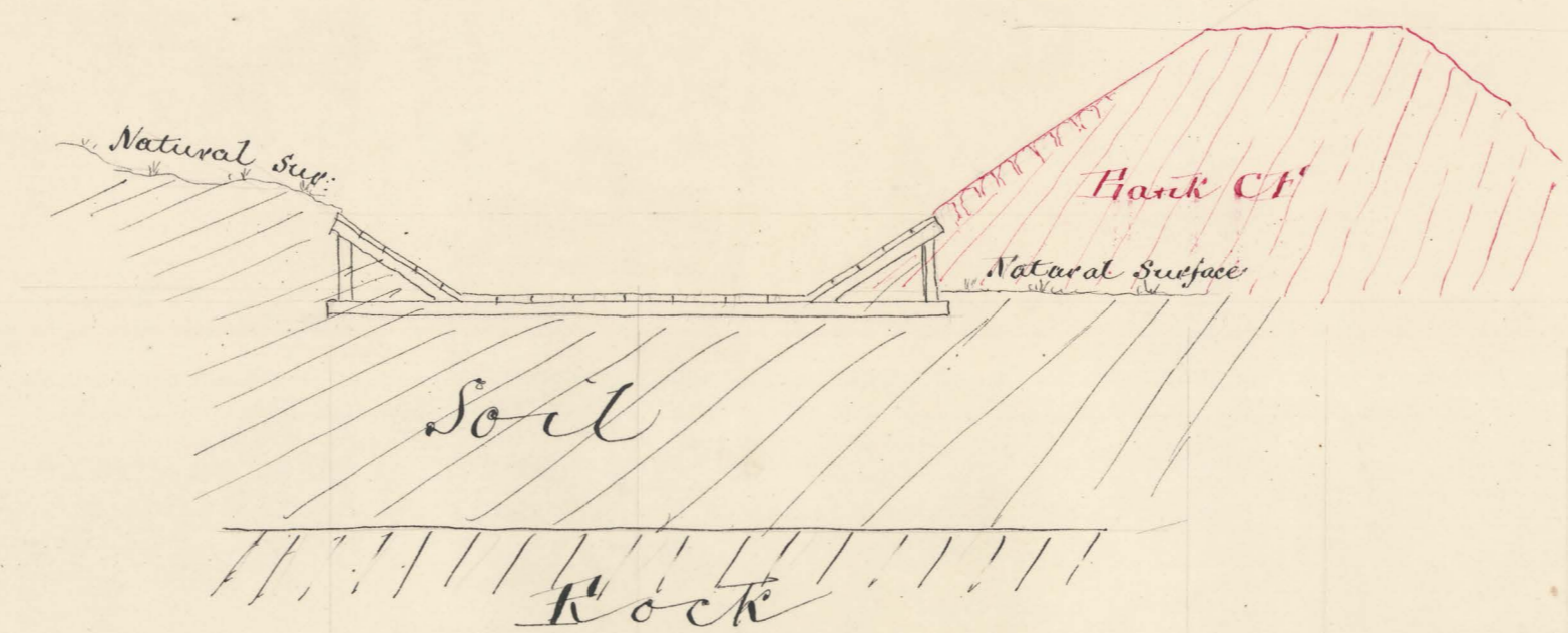
Cross Section at C
