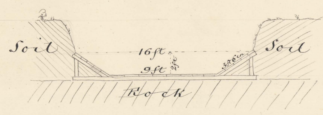
Cross Section at D
