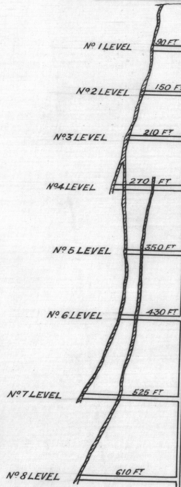
CROSS SECTION THROUGH CHUM MAIN SHAFT.
