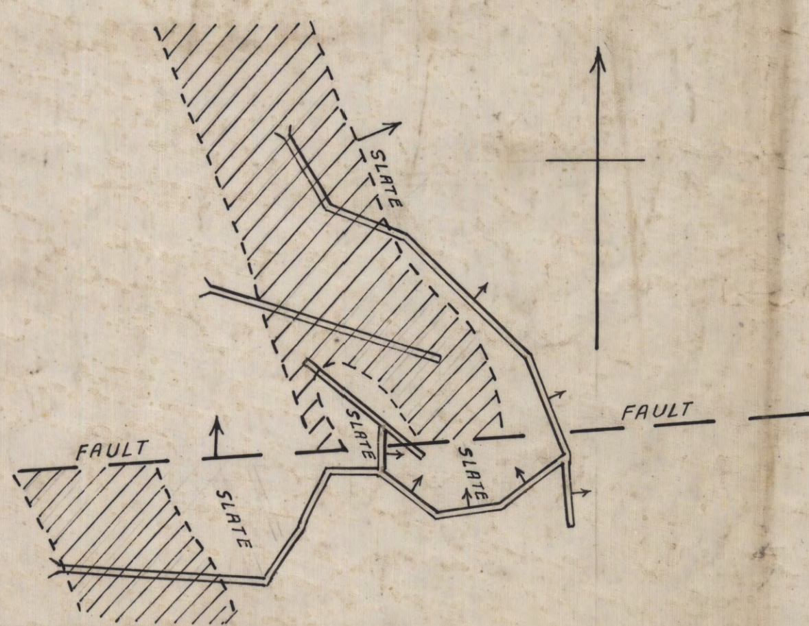
PLAN SHOWING FAULTING OF LODE
