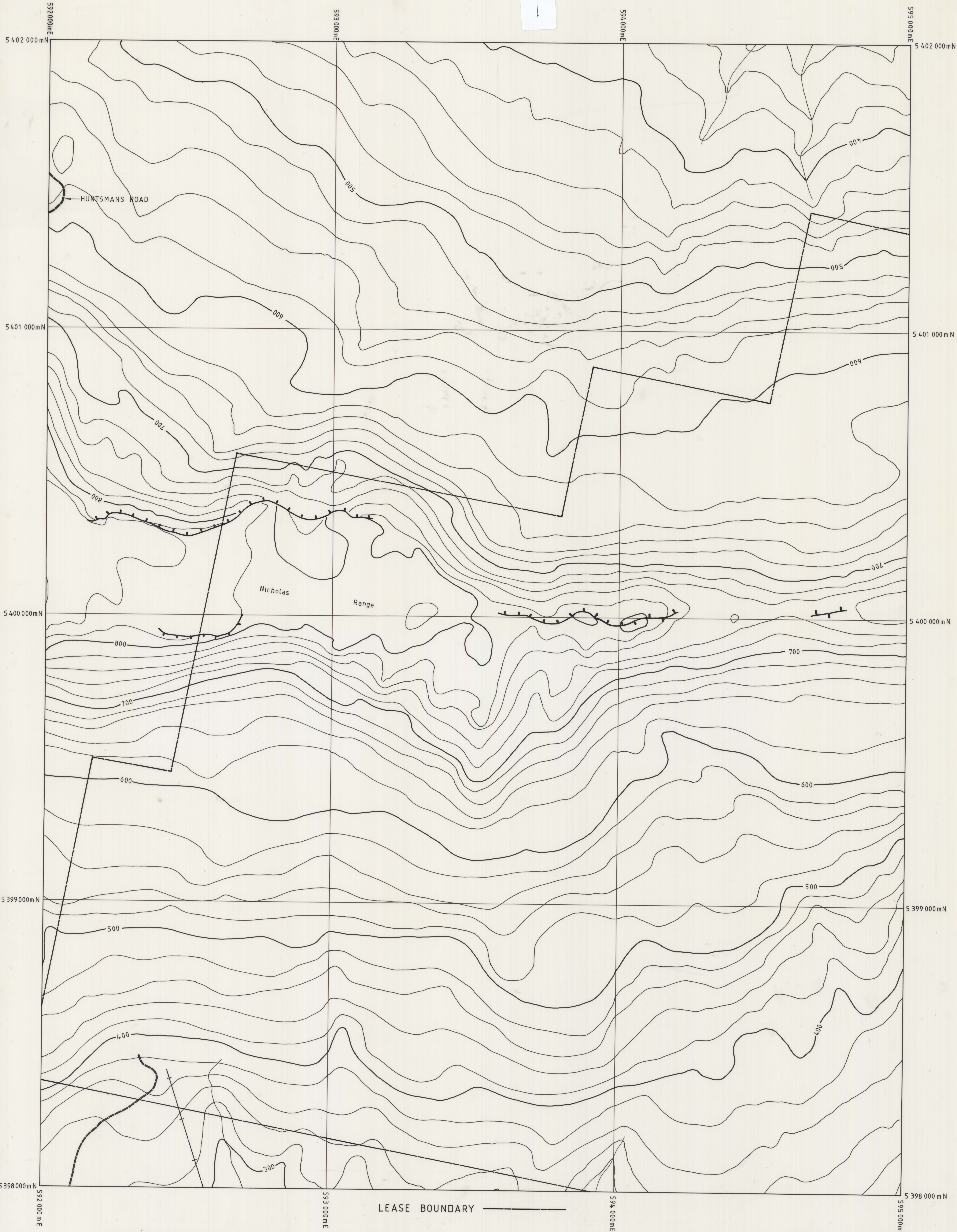
TOPOGRAPHIC BASE BLACKWOOD COLLIERY Drawn 22/9/83 - Scale 1:5000 - Department of Mines PLAN 353
