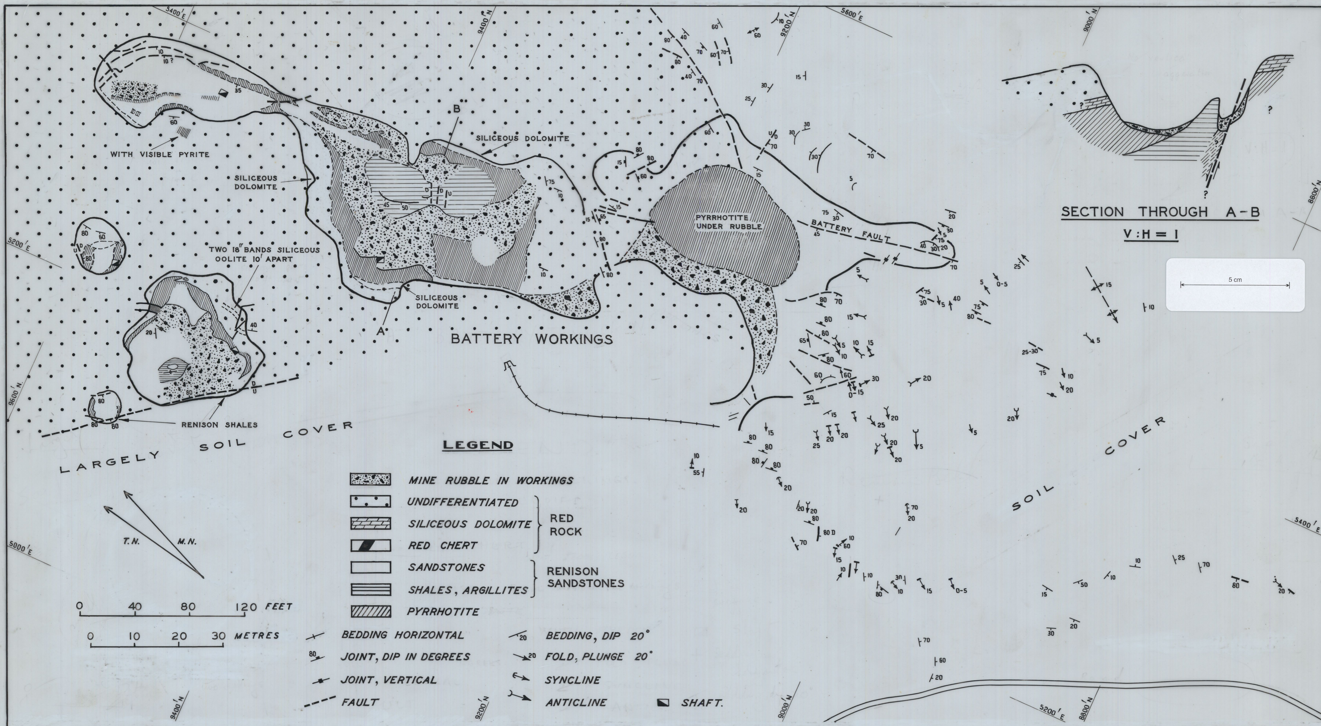
GEOLOGY—BATTERY WORKINGS, RENISON BELL GEOLOGY BY P.A. HILL AND M. SOLOMON, 1961.
