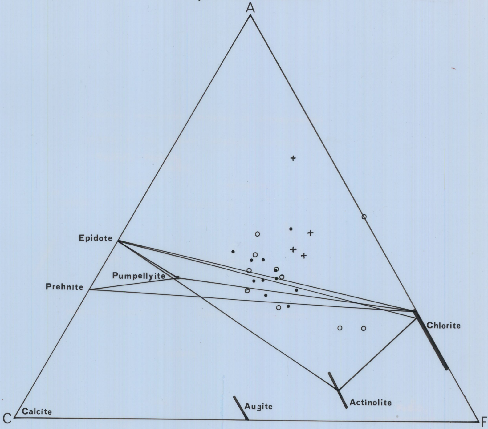
A~F plot of massive; altered, and "adjusted" basalt compositions
