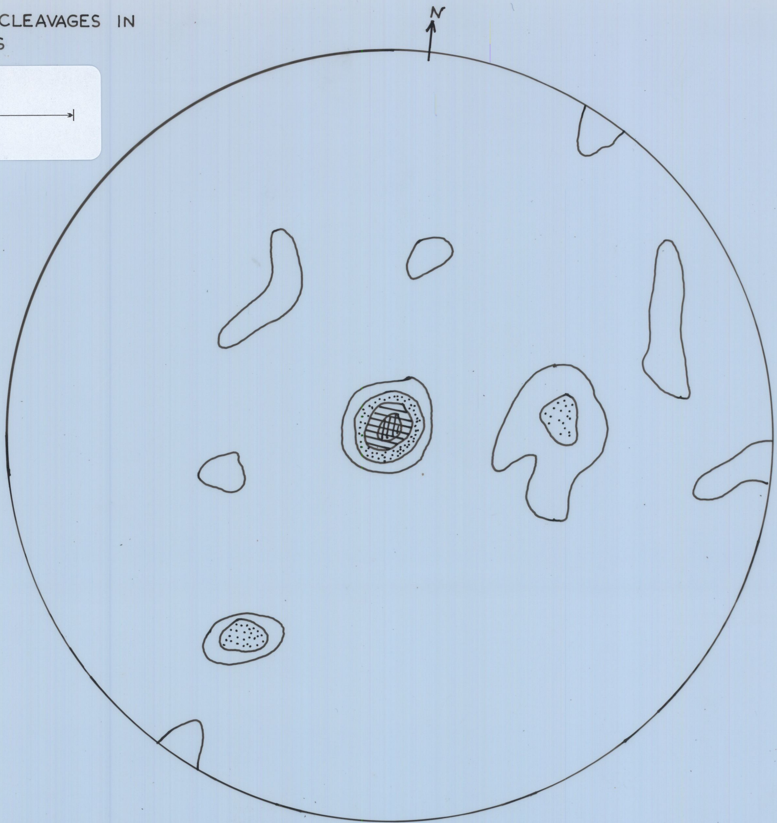
POLES TO THE FAULT PLANES, EQUAL ANGLE LOWER HEMISPHERE PROJECTION CONTOUR INTERVAL = 2%
