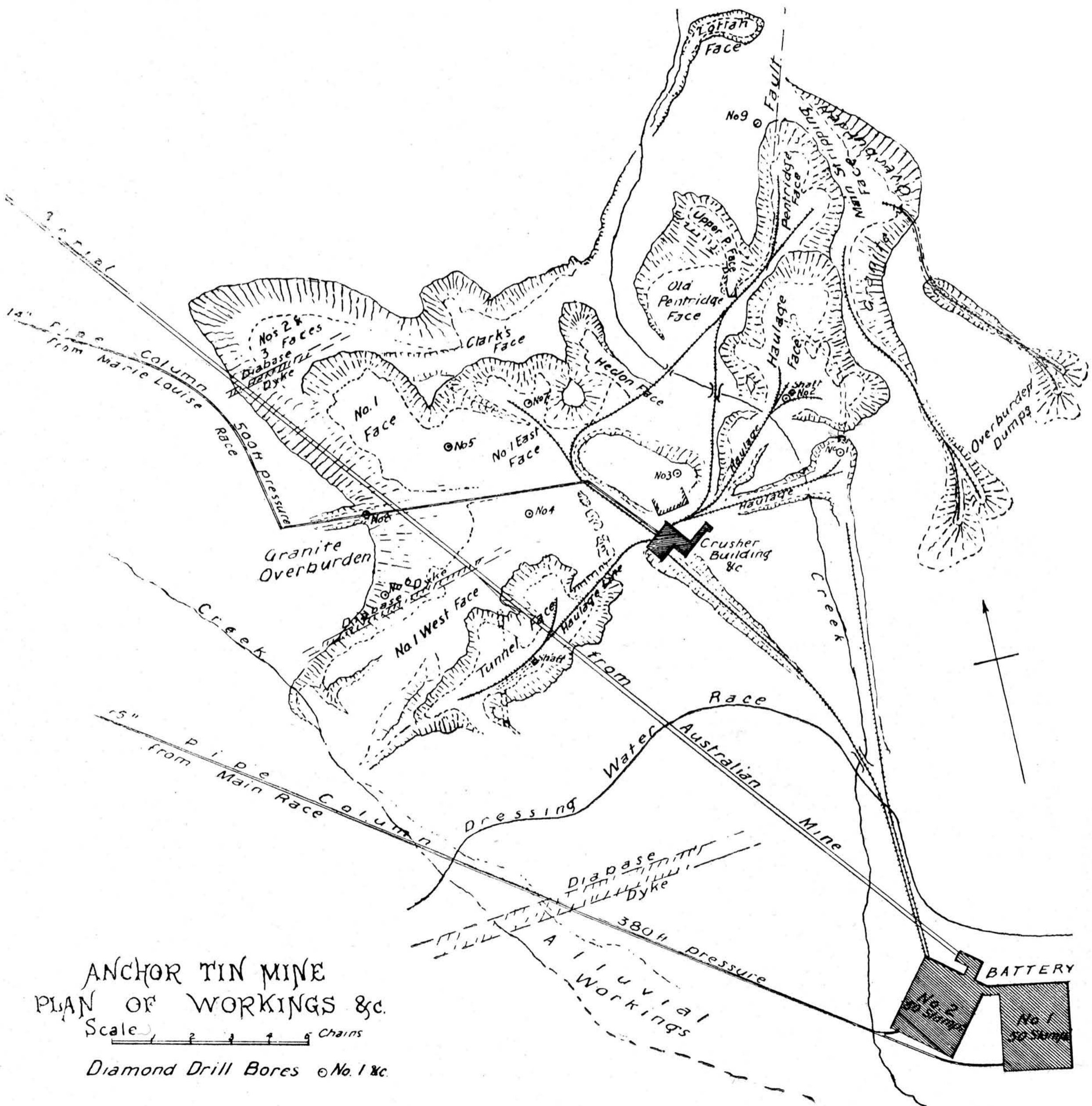
Fig. 1. Plan of Anchor Tin Mine Workings
