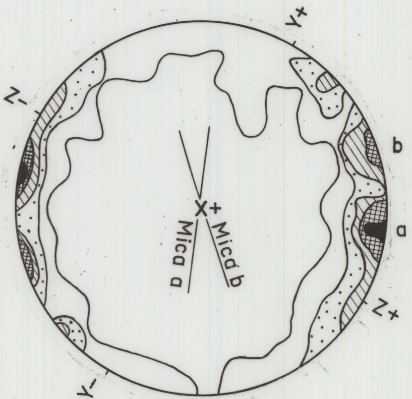
(g) 200 MUSCOVITE 9, 7, 5, 3, 1%
