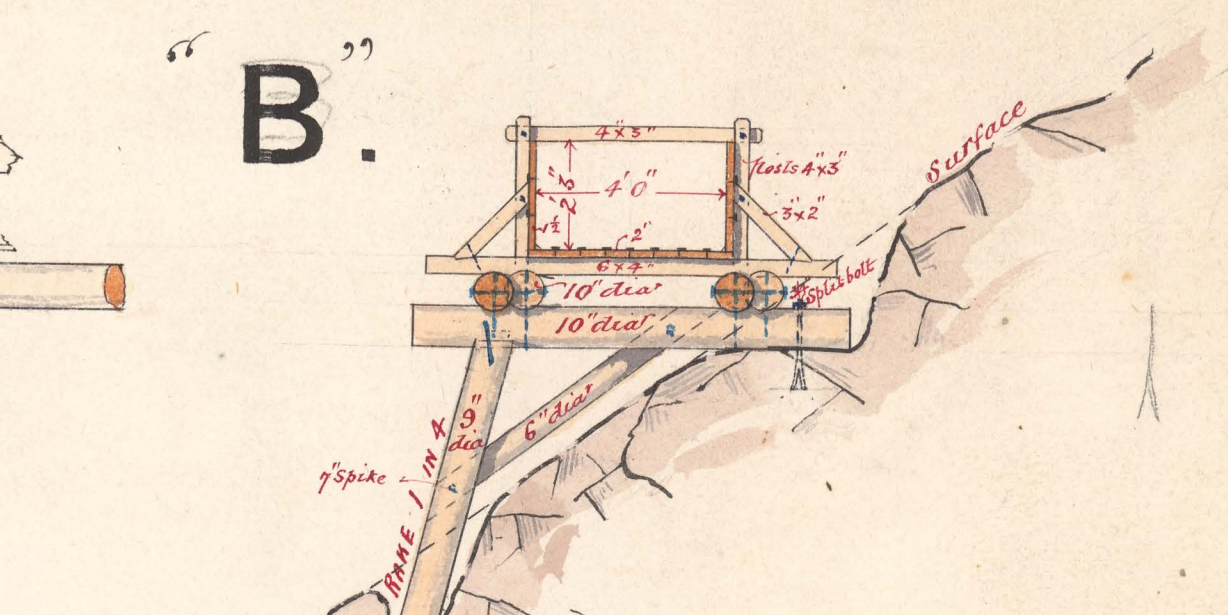
CROSS SECTION.
