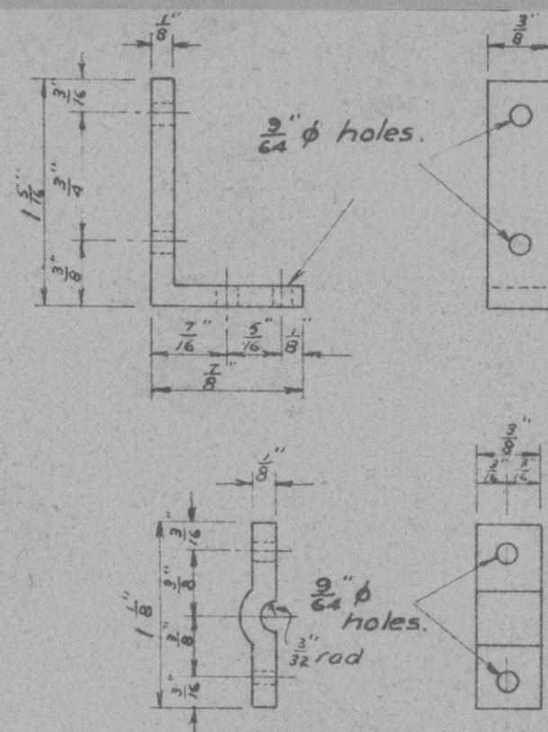
— CABLE FASTENER BRACKET —
