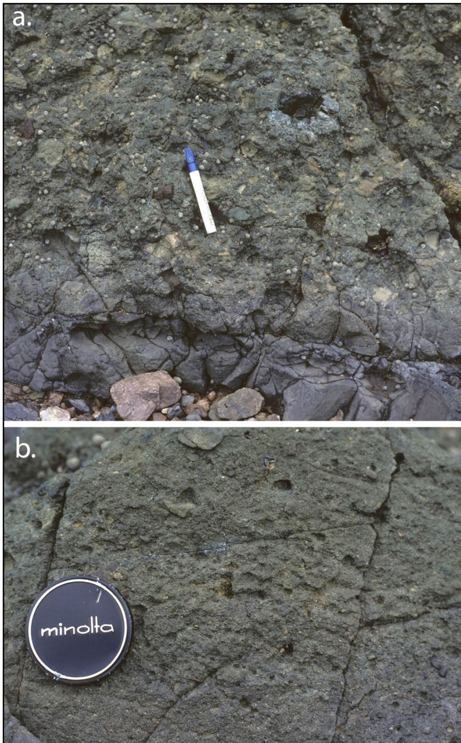
Figure 17. Mudstone and lithic wacke lithologies of the Beecraft Megabreccia, Penguin foreshore. a) Mudstone-matrix-supported conglomerate (sedimentary "breccia") transitional into bedded mudstone. b) Coarse, sandy lithic wacke with occasional, small pebble-sized clasts/fragments.
