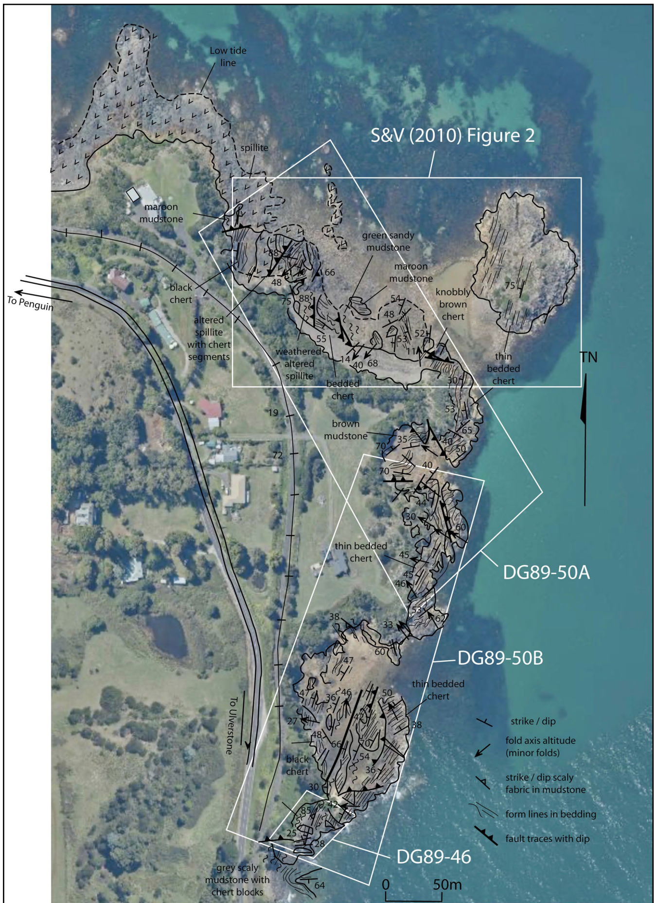
Figure 27. Structural form line map of Loders Point superimposed on Google satellite image. Formlines in bedding S_0 are shown by the black line traces. Mapped areas are shown by the white rectangular polygons including the detailed mélangé map of Seymour and Vicary (2010, fig. 2), and detailed field sketch maps labelled DG89-46, DG89-50A and DG89-50B (see Appendix 2).
