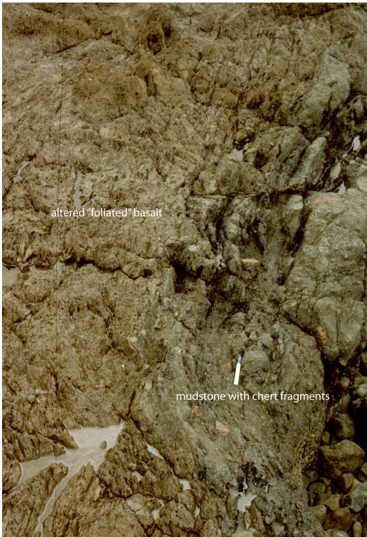
Figure 30 (Left). Contact between altered, foliated basalt and fissile, foliated mudstone with chert clasts at the western end of the mélangé.
