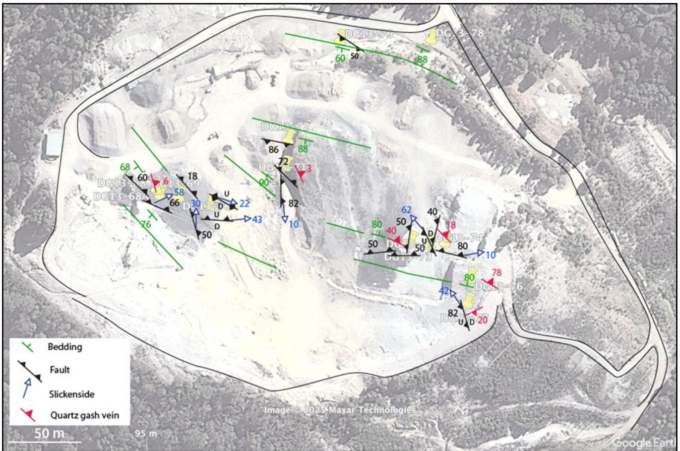
Figure 54. Structural map of the Shackley Hill quarry on Google satellite image base. Form lines in bedding are shown by the green line traces. Quartz gash vein sets (red strike/dip symbols) tend to have a NW-strike and a moderate to gentle NE-dip. Compare the fault traces with the sketch-mapped faults in Figure 57.
