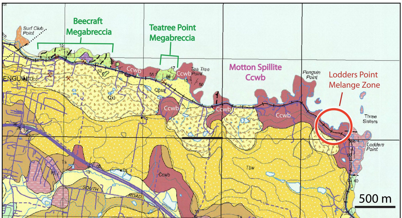
Figure 14. Penguin Luina slice lithological components exposed in coastal outcrops between Penguin and Lodders Point. Map Base is from the MRT digital atlas 1:25 000 series. The slice largely consists of basalt (Ccwb/Motton Spillite) with zones of sedimentary megabreccias and a large block of chert at Lodders Point. The megabreccias include: the Beecraft Megabreccia and the Teatree Point Megabreccia. The Lodders Point mélangé is a foliated interface between the basalt and the large chert block.
