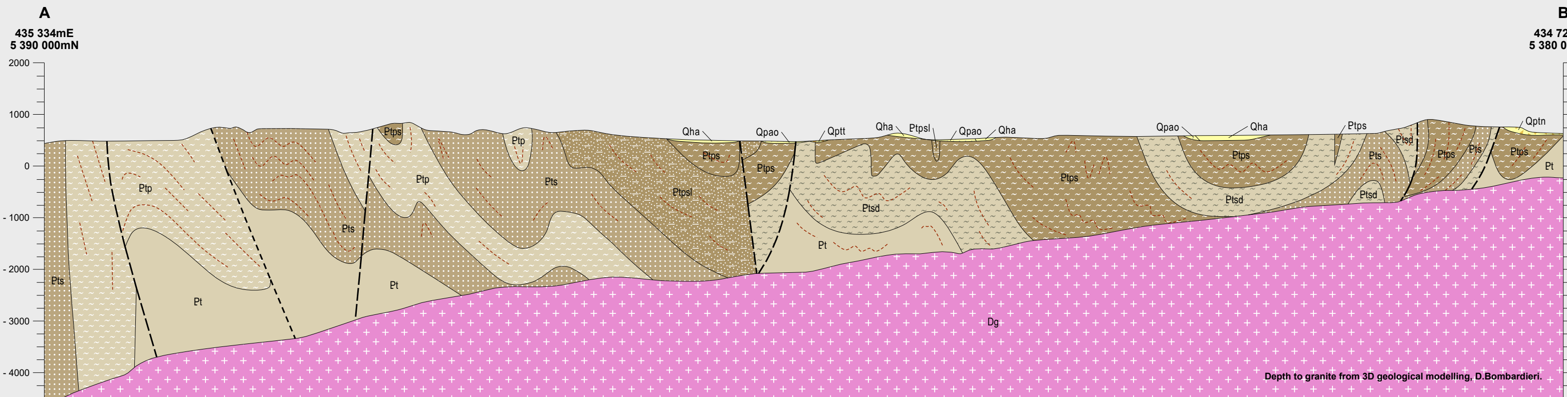
SECTION V:H = 1:1
