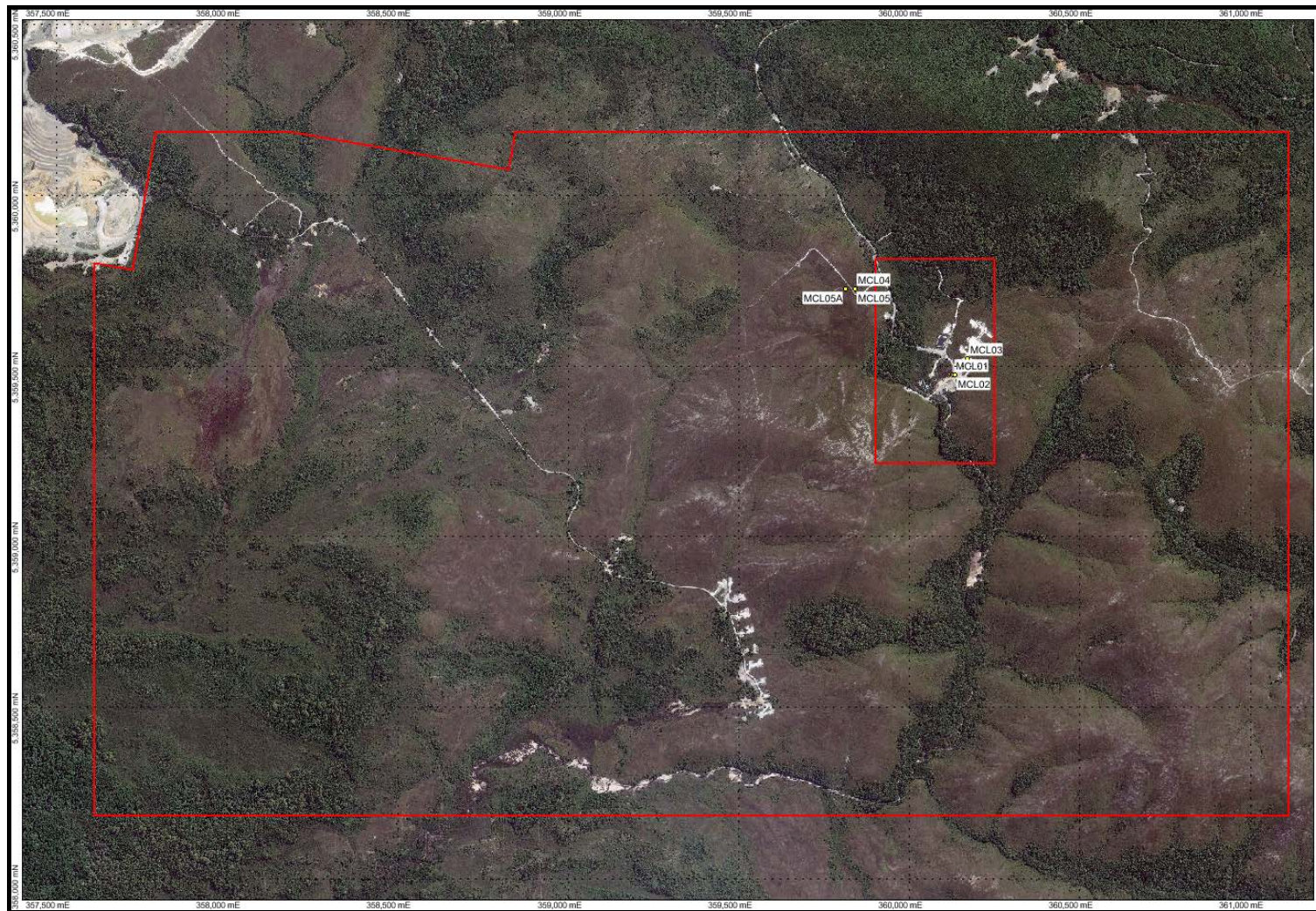
Figure 12 Plan of RMG Drill sites
