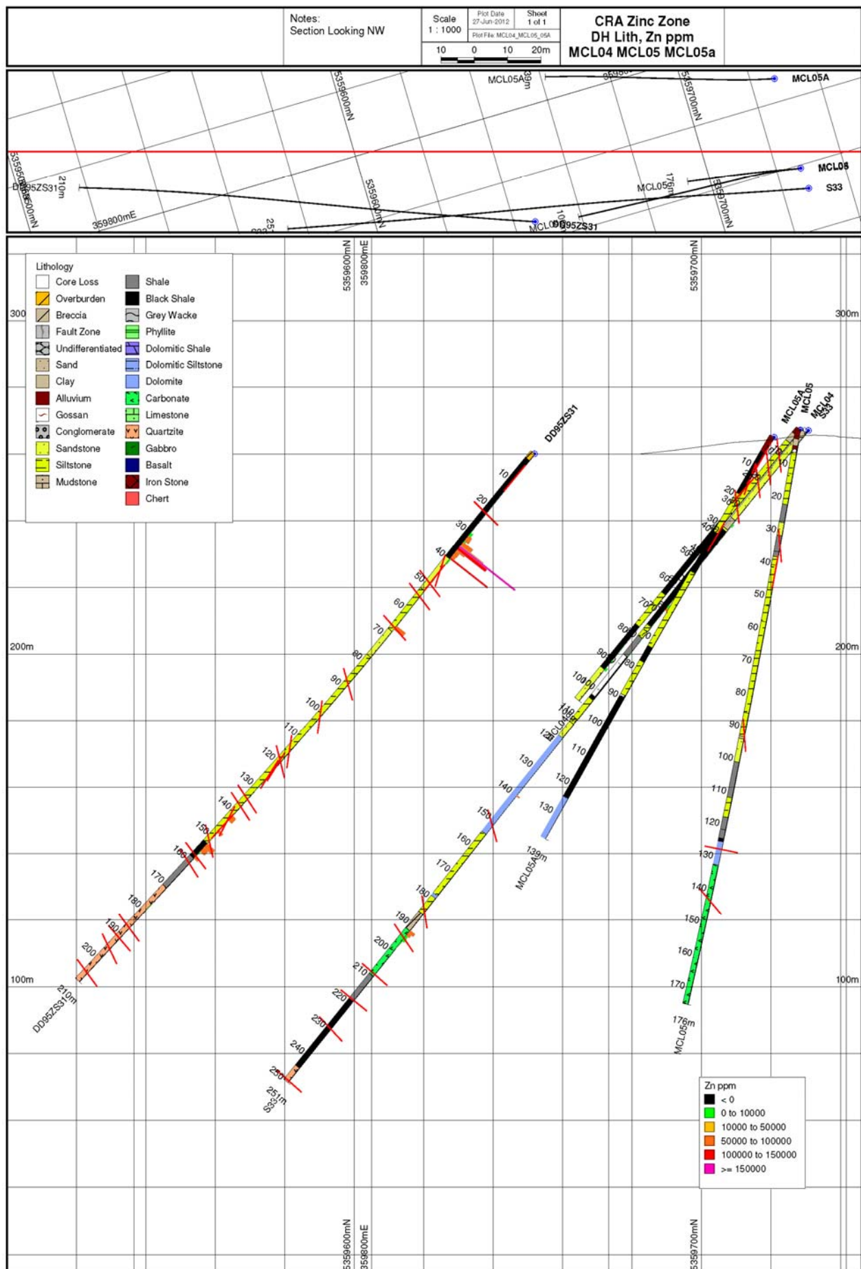
Figure 14 Cross section of drill holes at CRA zinc zone
