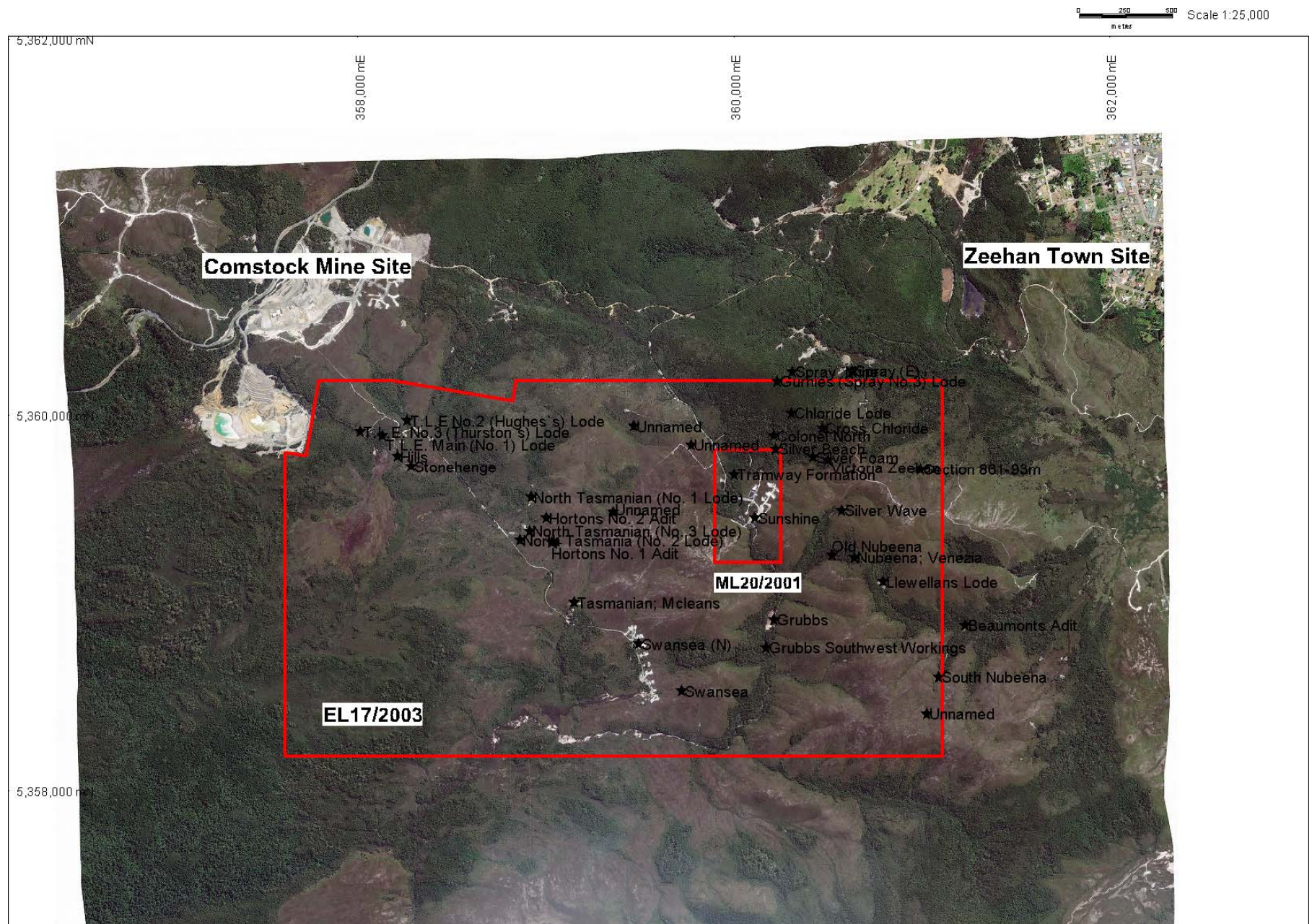
Figure 2 Historical zinc-lead prospects
