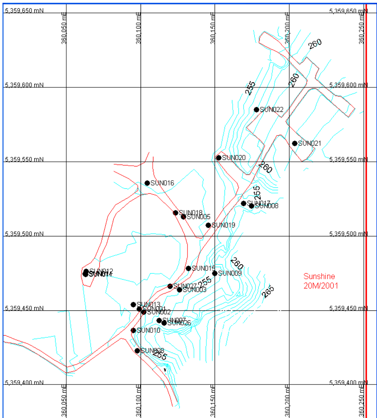
Figure 7 Plan of Stonehenge Sunshine drill holes
