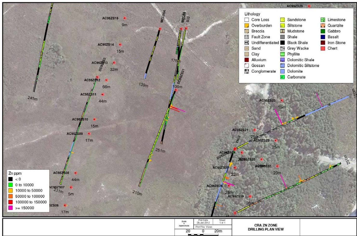
Figure 13 Plan of all holes at CRA zinc zone
