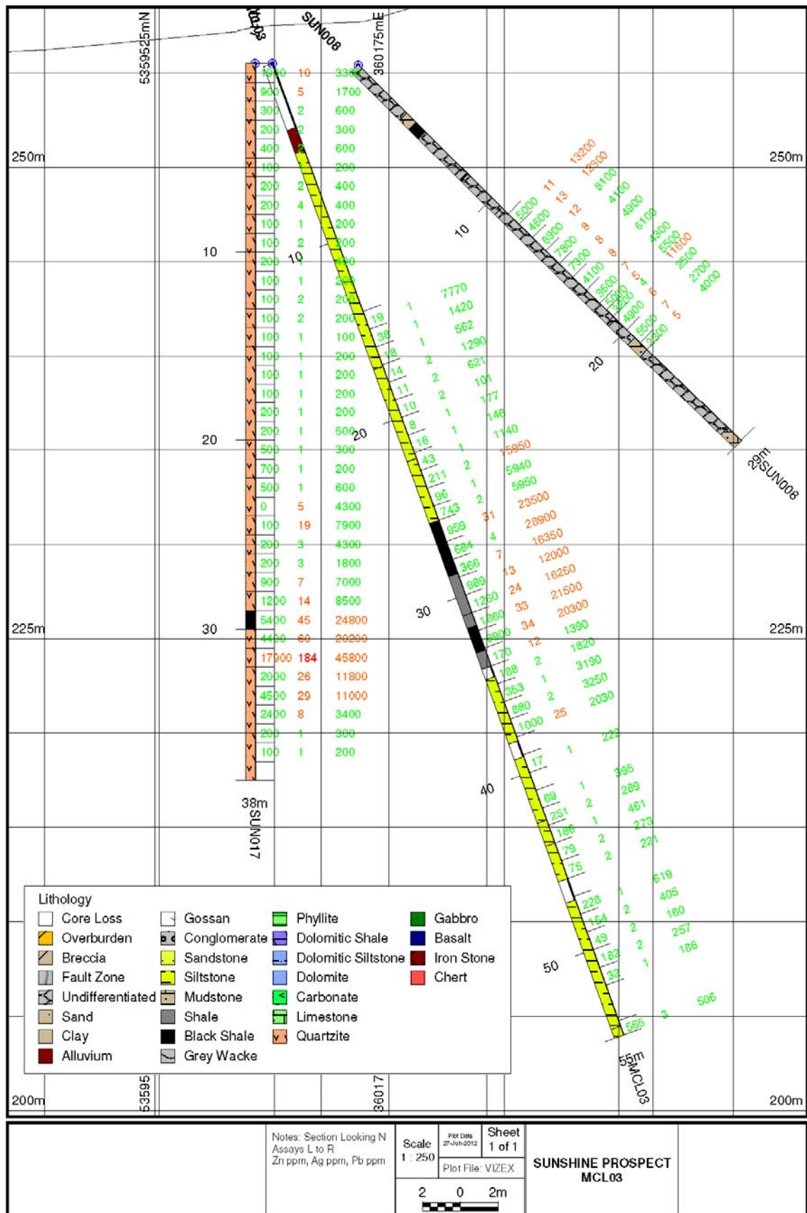
Figure 17 Cross section Sunshine MCL03
