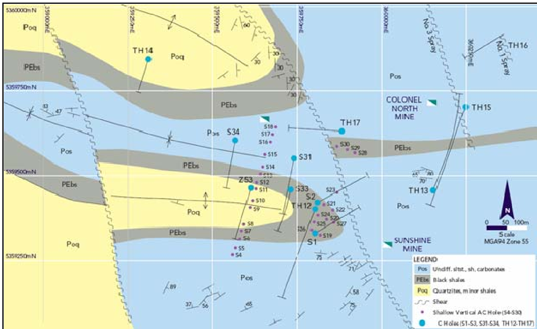
Figure 5 Plan of CRA and Renison drill holes
