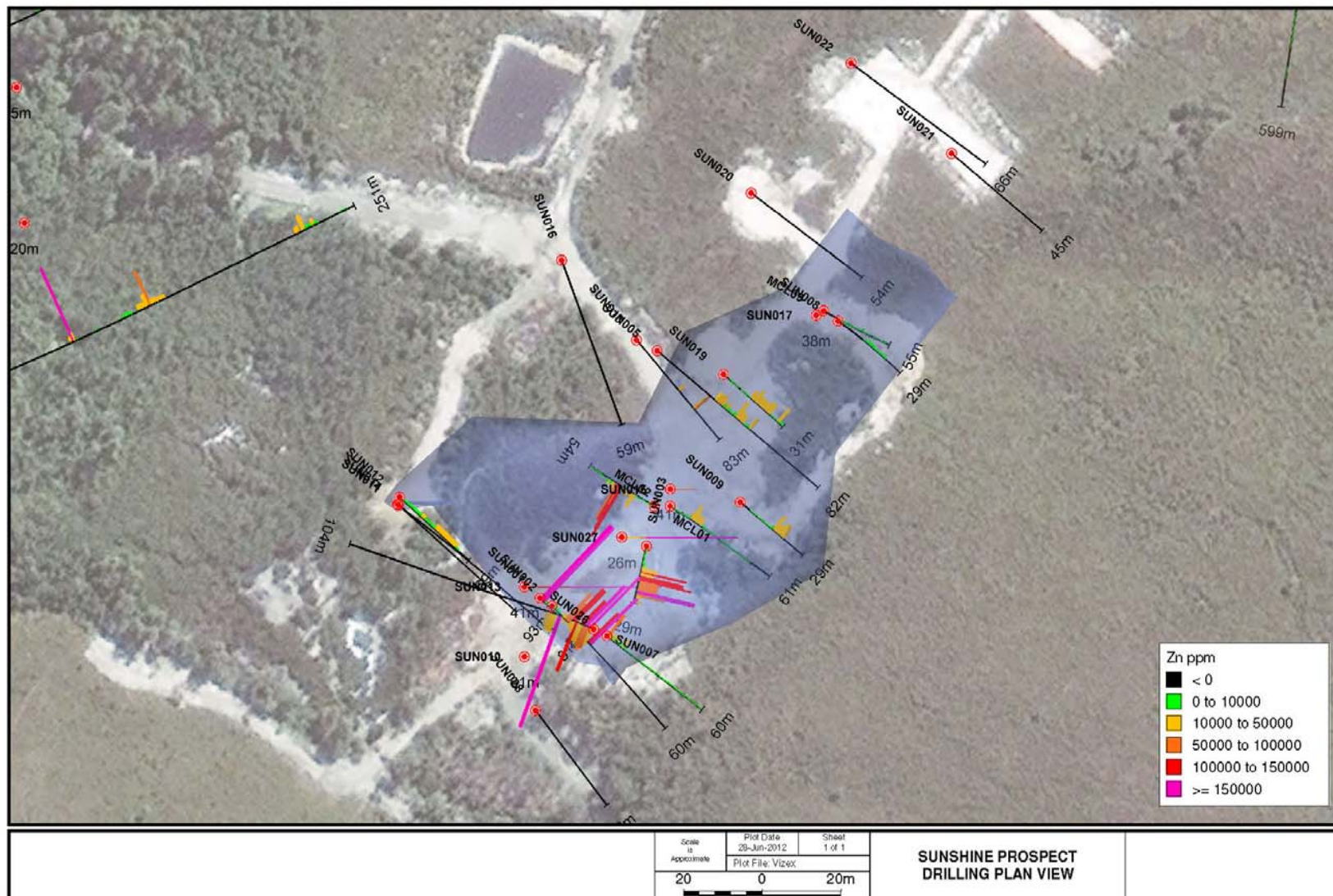
Figure 10 Plan of RMG Sunshine drill holes
