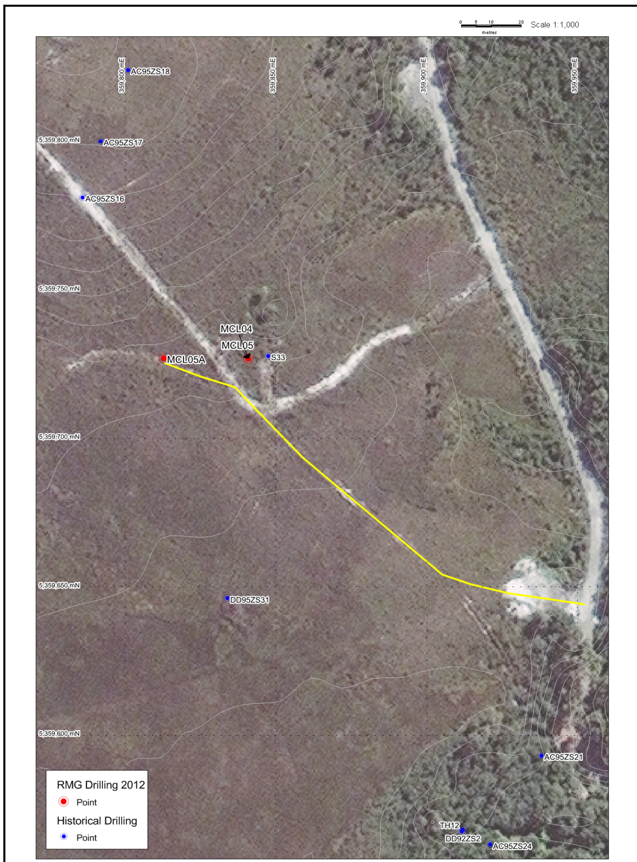
Figure 11 Plan of RMG drill holes at CRA Zinc zone
