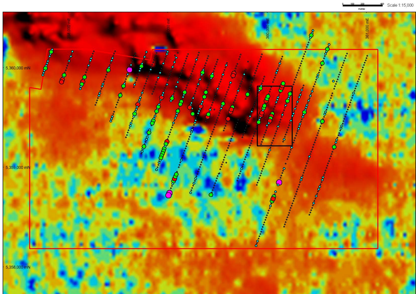
Figure 9 Plan of AEM anomaly and Renison soil geochemistry
