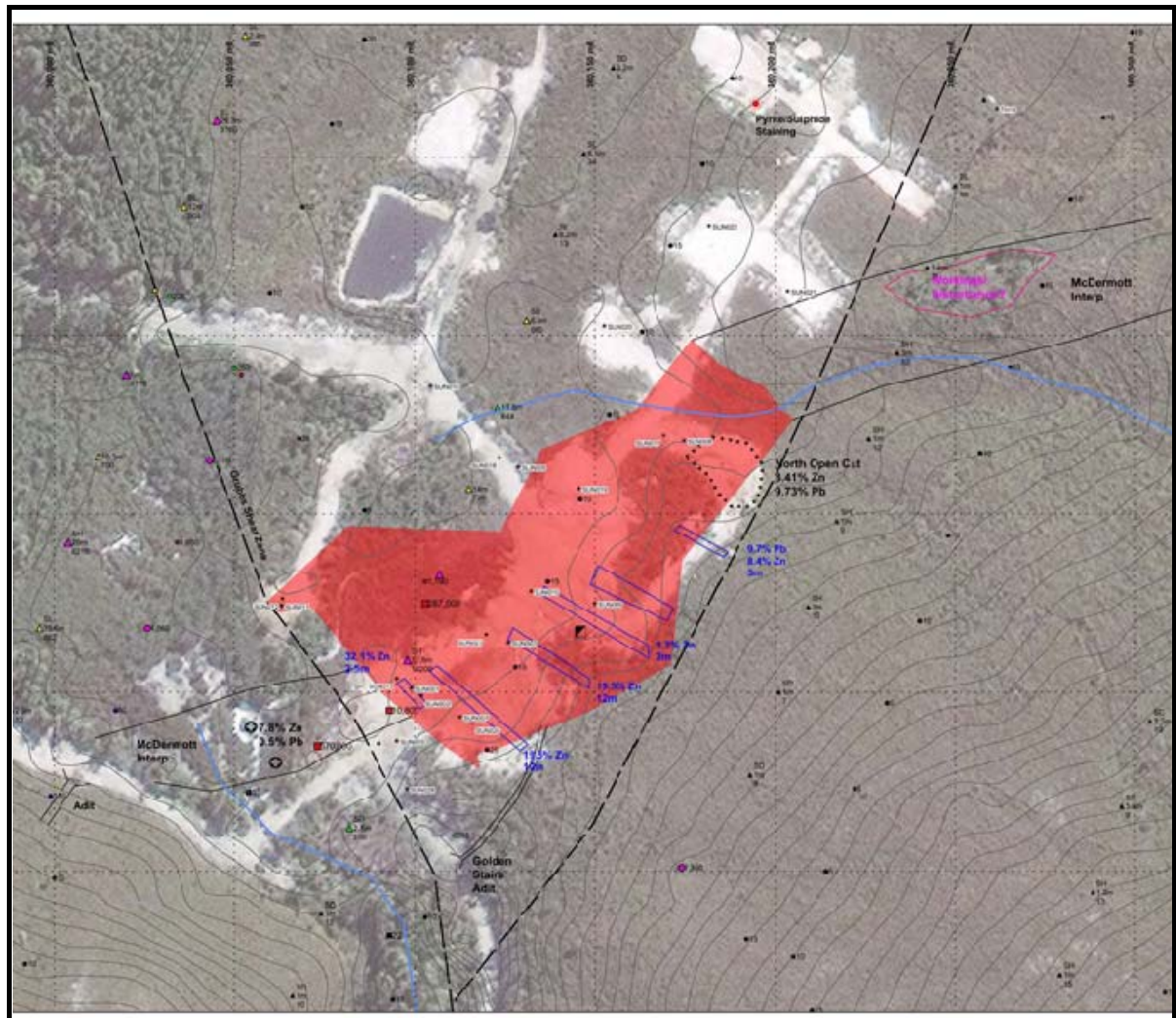
Figure 18 Plan of McDermotts trends at Sunshine
