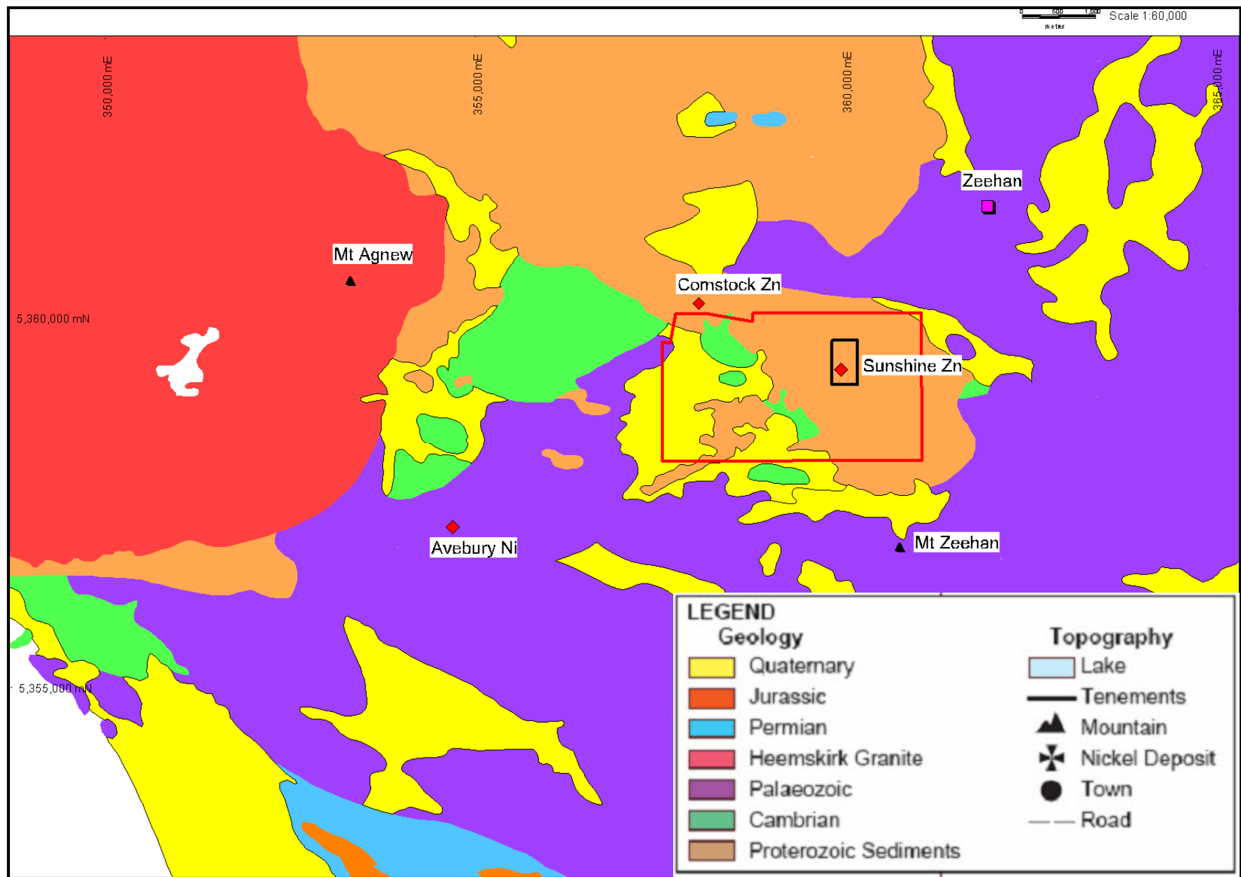
Figure 1 Regional geology and location of Licences
