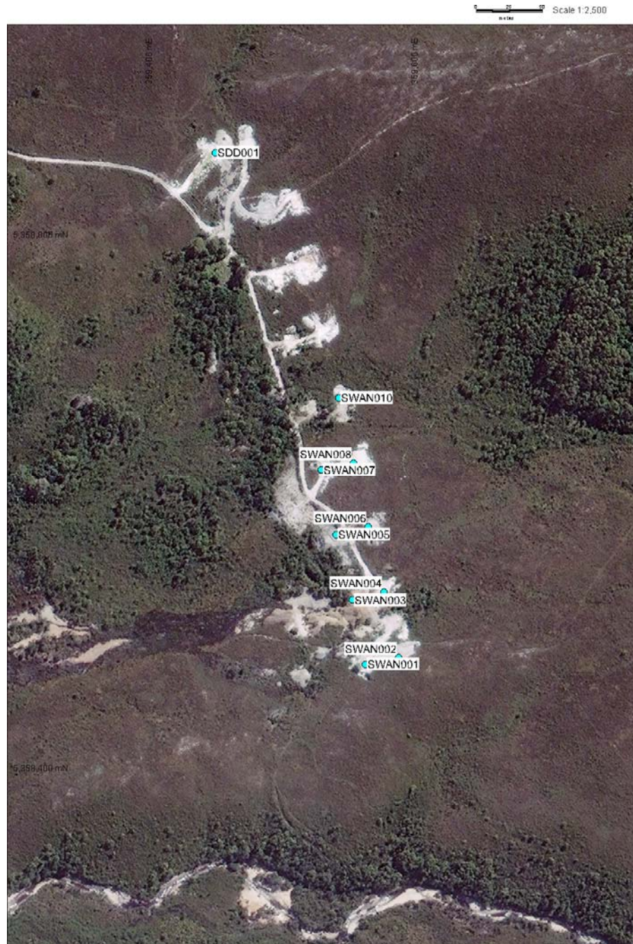
Figure 8 Plan of Stonehenge Swansea drill holes
