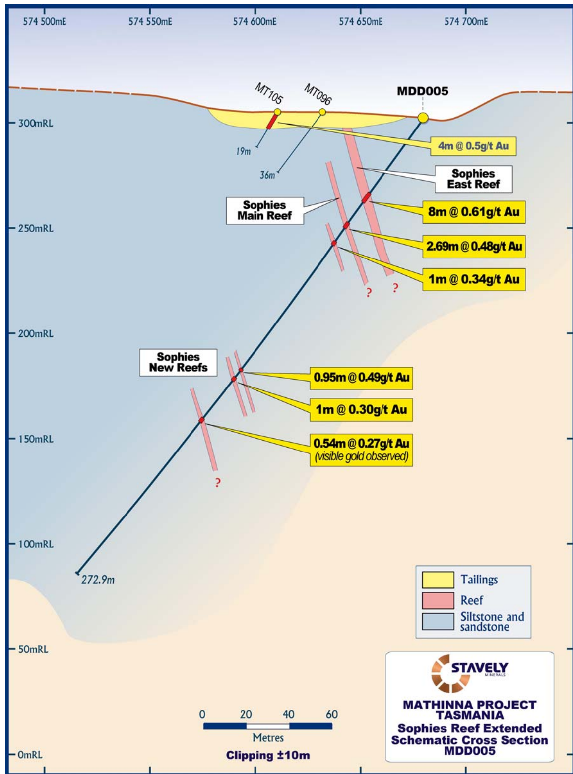
Figure 11. Sophies Reef Extended – Schematic Cross Section MDD005.
