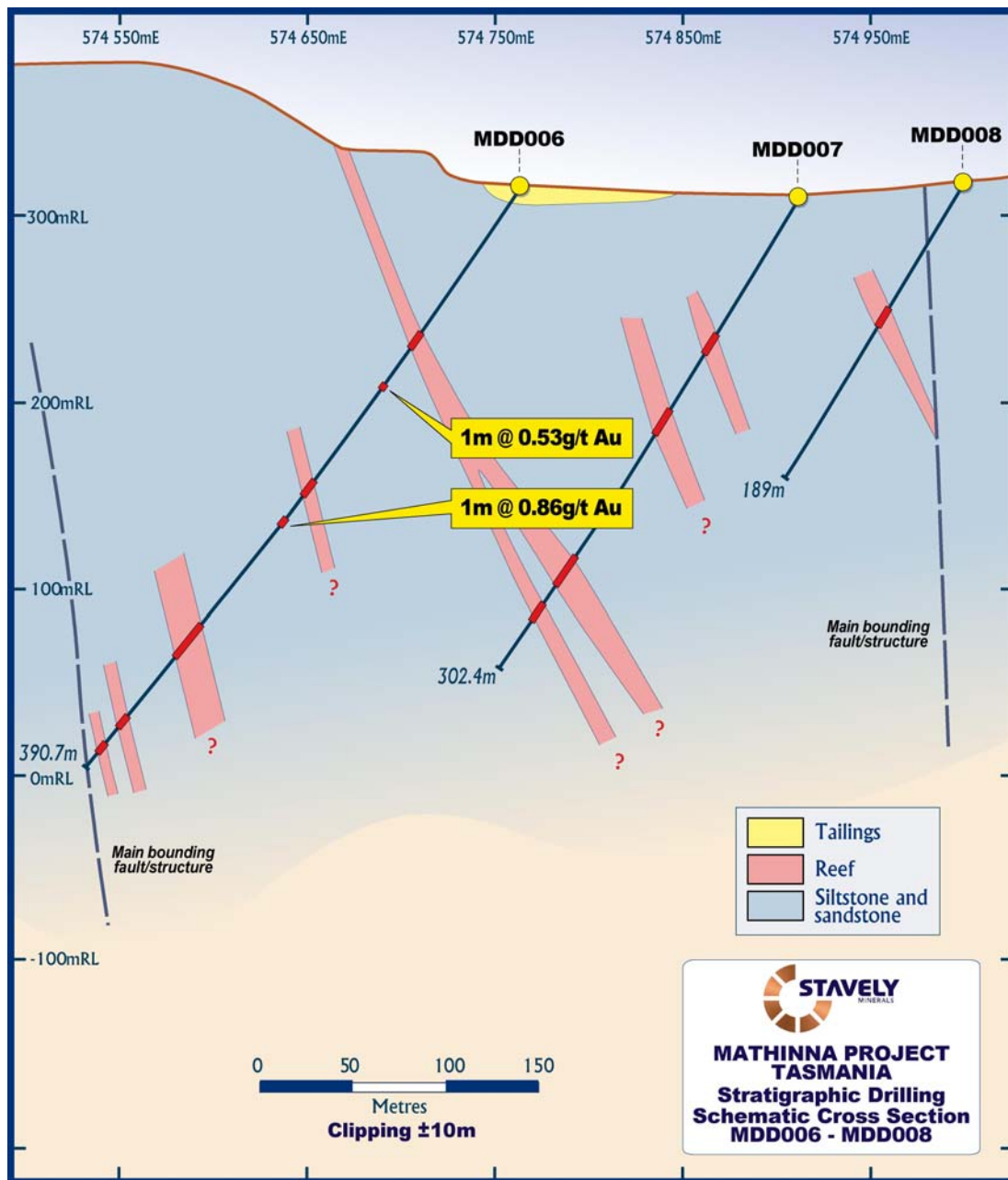
Figure 12. Stratigraphic Drilling Schematic Cross Section MDD006 – MDD008.
