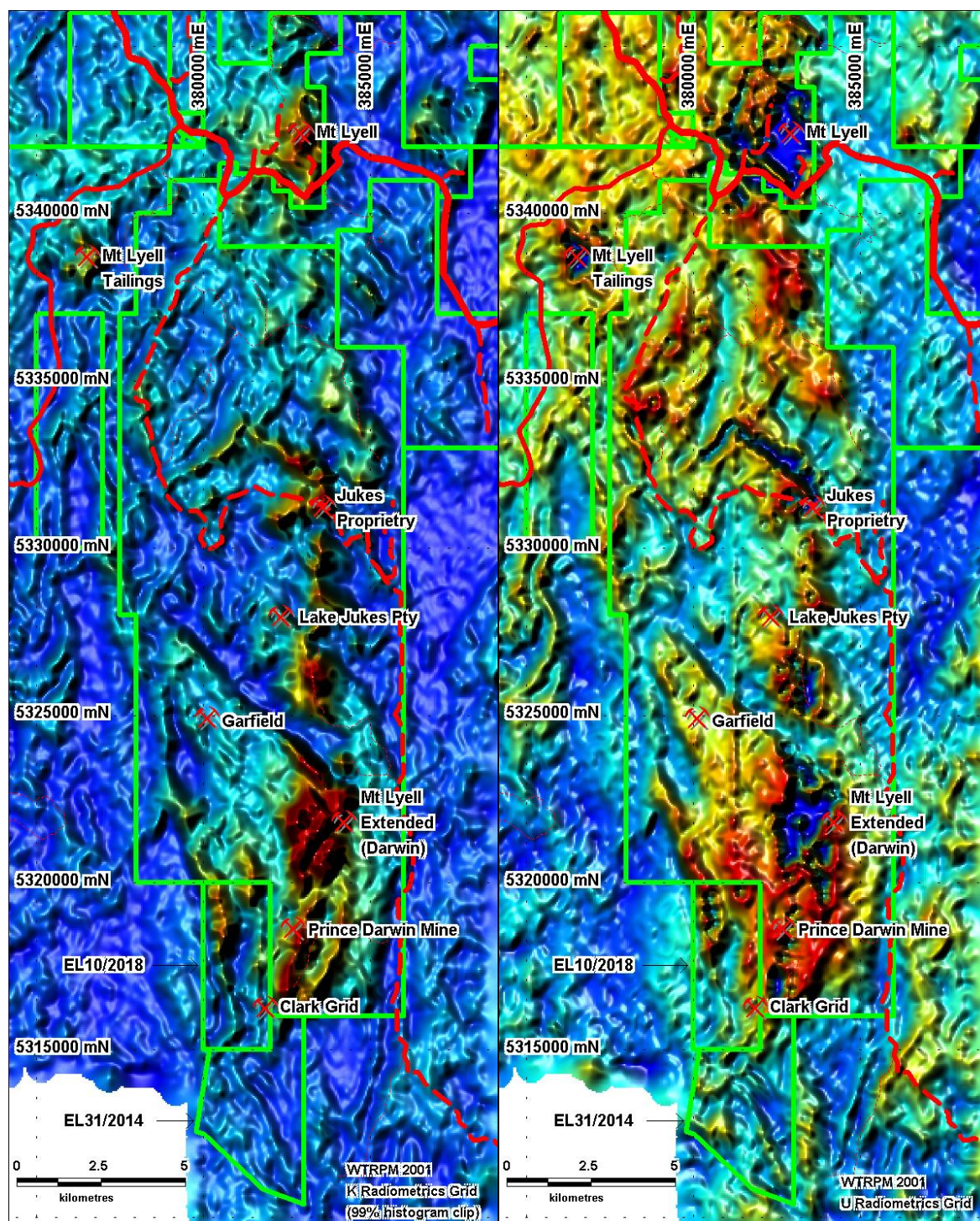
Figure 7: K (left) and U (right) Radiometrics grids displaying 99% histogram clip to highlight significant highs and lows; Regional view from Mt Lyell extending south through EL10/2018.
