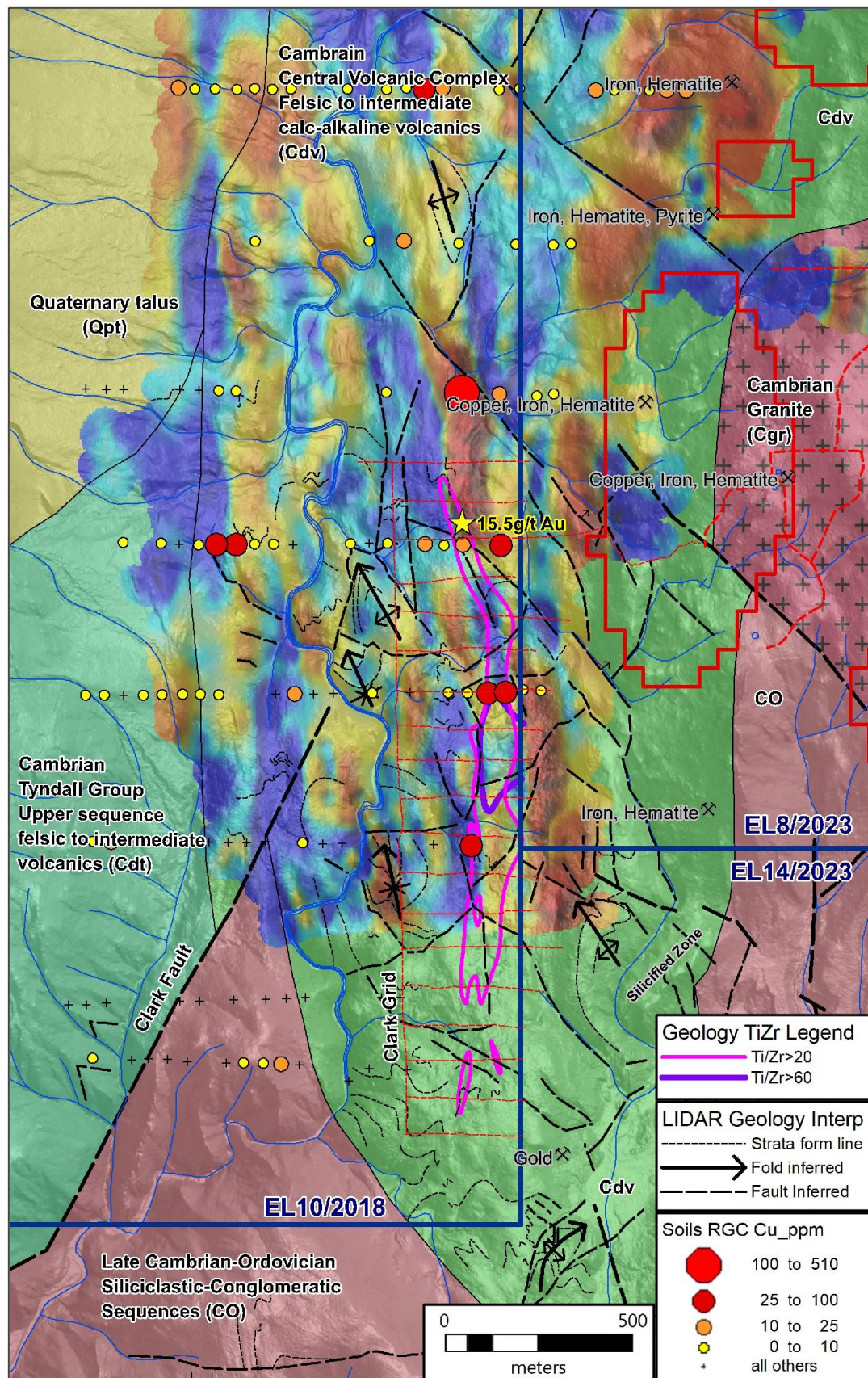
Figure 11: Regional 250k scale geology overlay by IP chargeability grid and LIDAR DTM transparency, highlighting salient prospective features of EL 10/2018 and surrounds (Andesitic VHMS host horizon (Ti/Zr>20), RAI contours in red)
